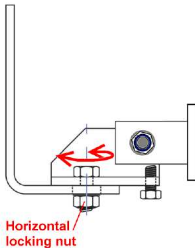
Fig 6.3-4 Horizontal swivel
