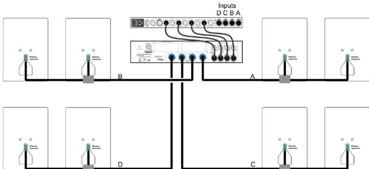
Fig 9.4-8 4-channel 4 ohm patch using Funktion One XO4A controller and F40Q amp (4 x 2-way configuration shown, F81s with Phoenix connectors)
